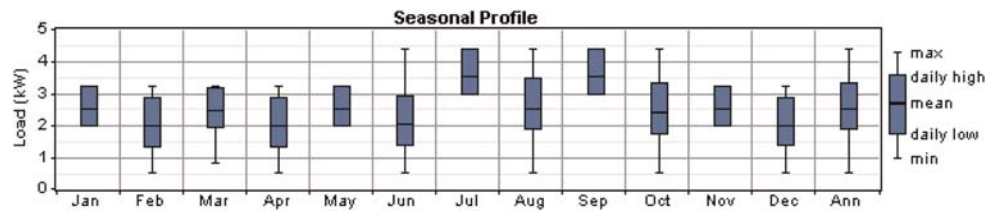
Figure 1. Load profile for poultry house (without-DSM).
