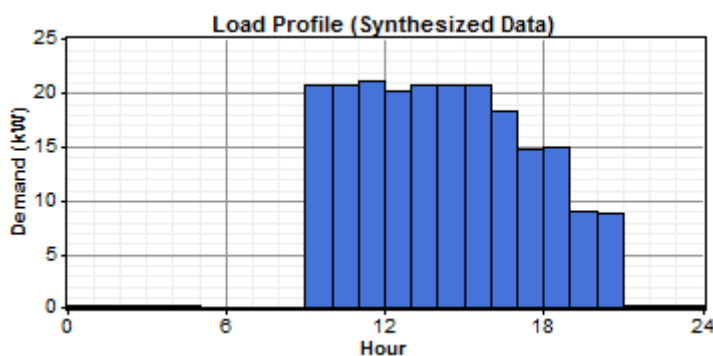
Fig. 4: Load profile of primary load 2
