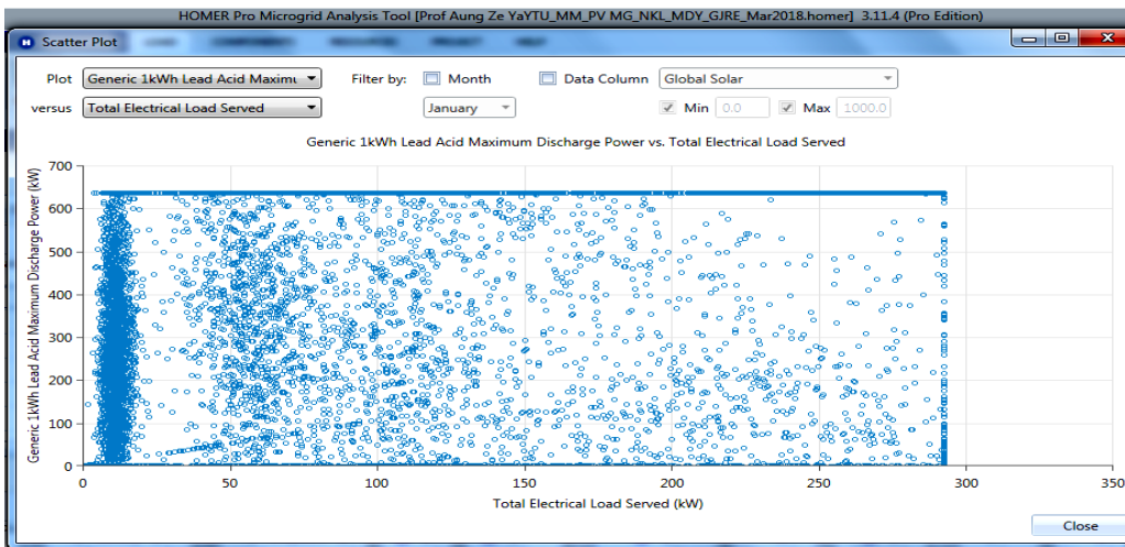
Fig. 36: The Battery Discharge vs. Total Electrical Load Served of Proposed PV Mini-Grid (100% RE)
